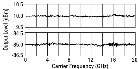
Typical output level accuracy and flatness at +10 and -85 dBm
